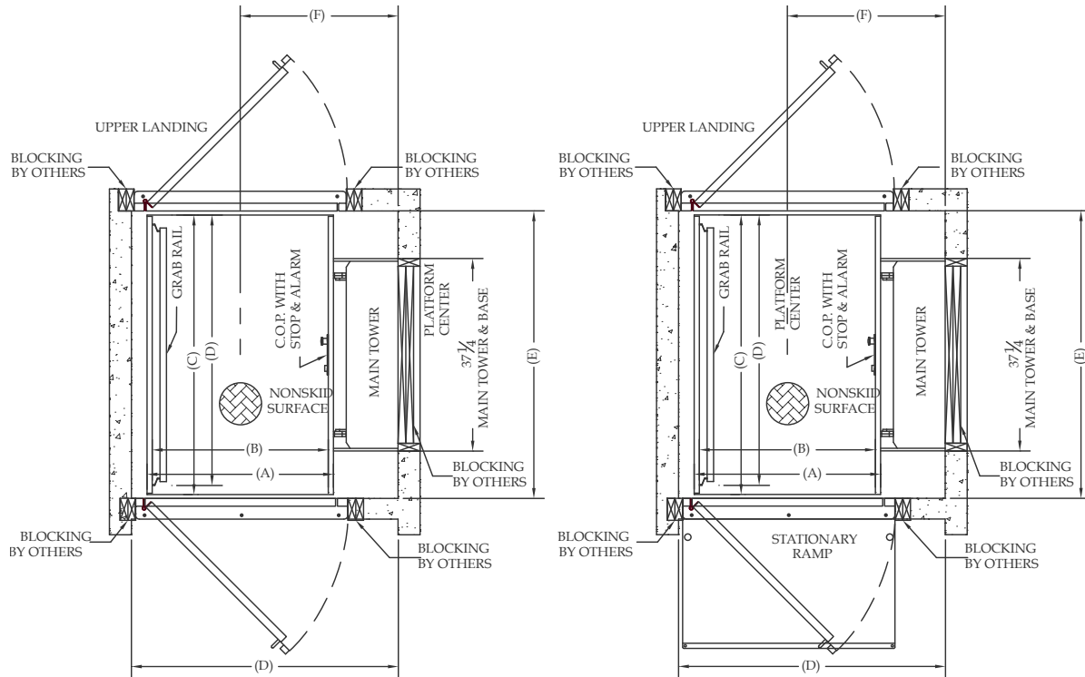
LOWER LANDING PIT MOUNTED APPLICATION SHOWN
